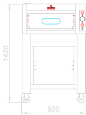
VISTA FRONTALE + SUPPORTO FRONT VIEW + STAND
